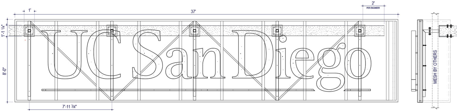
FRONT VIEW
